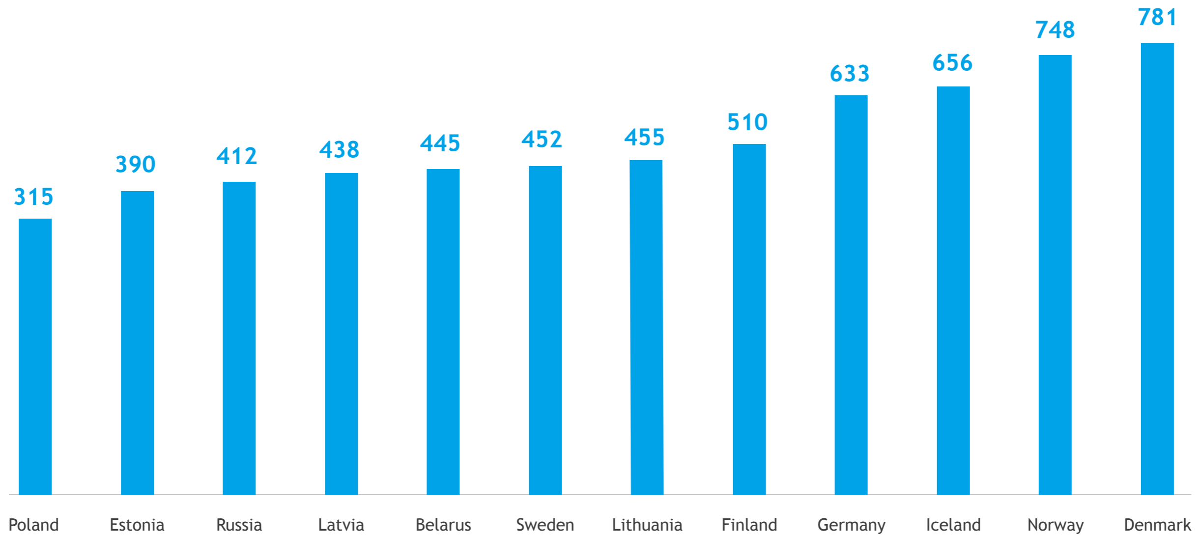
👁 CHART 7. GENERATION OF MUNICIPAL WASTE (KG PER CAPITA)
