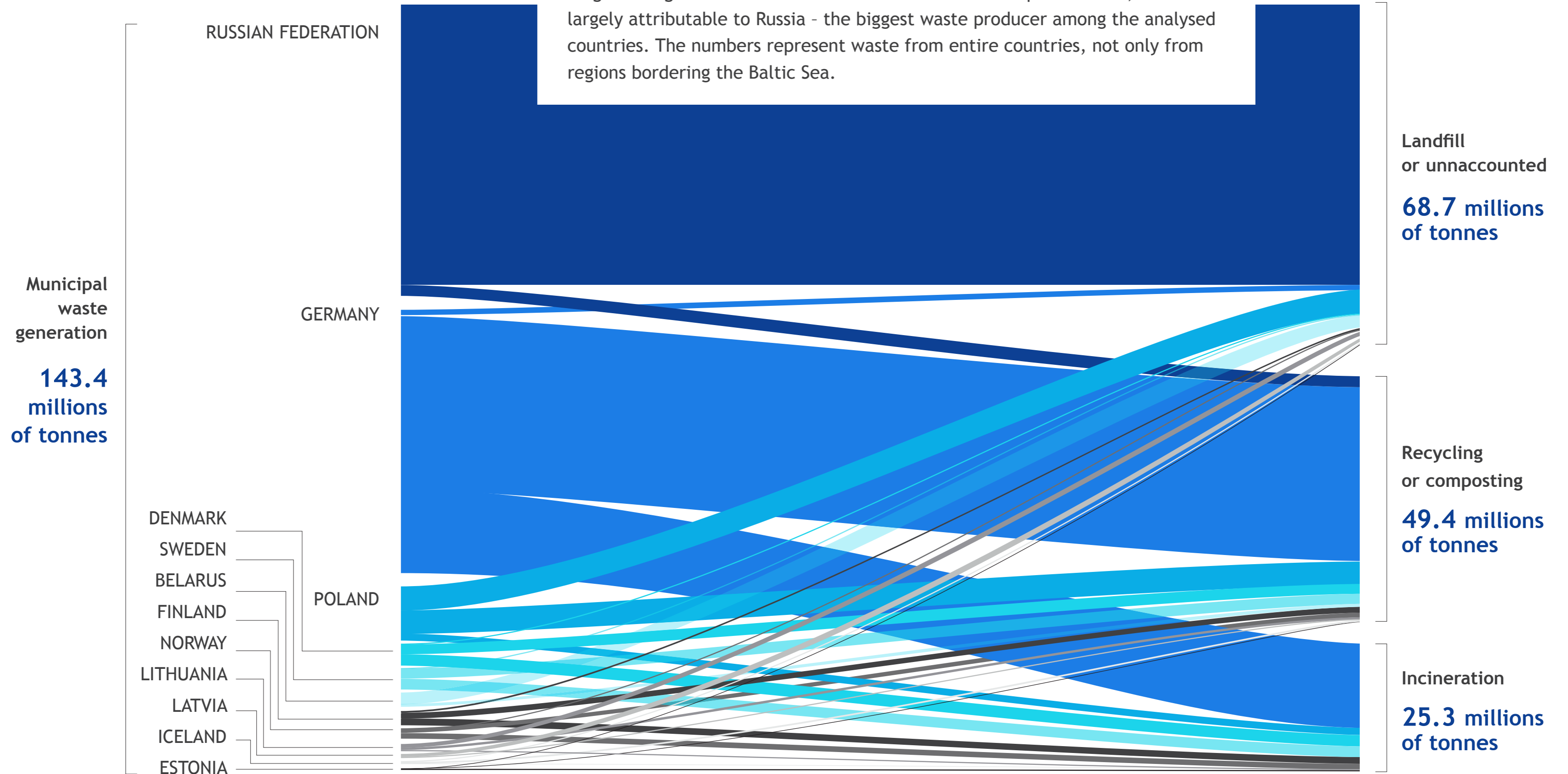
CHART 1. WHAT THE BSR COUNTRIES DO WITH THEIR MUNICIPAL WASTE?
