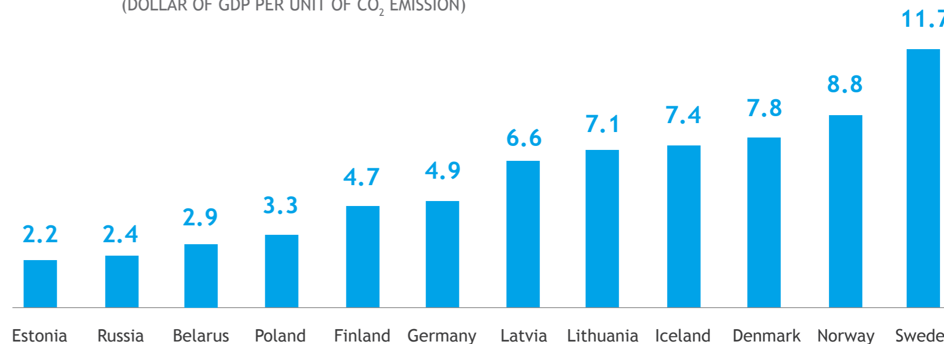
👁 CHART 5. PRODUCTION-BASED CO 2 PRODUCTIVITY (DOLLAR OF GDP PER UNIT OF CO 2 EMISSION)
