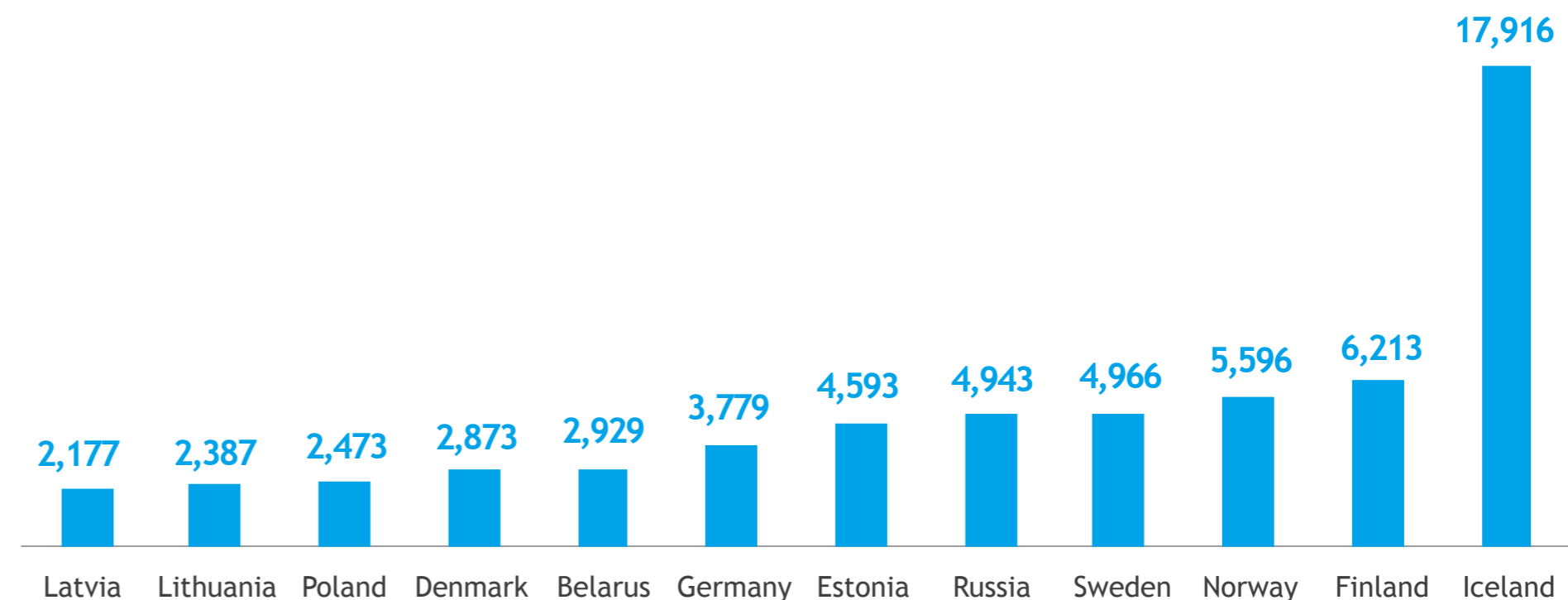
CHART 6. ENERGY CONSUMPTION (KG OF OIL EQUIVALENT PER CAPITA)
