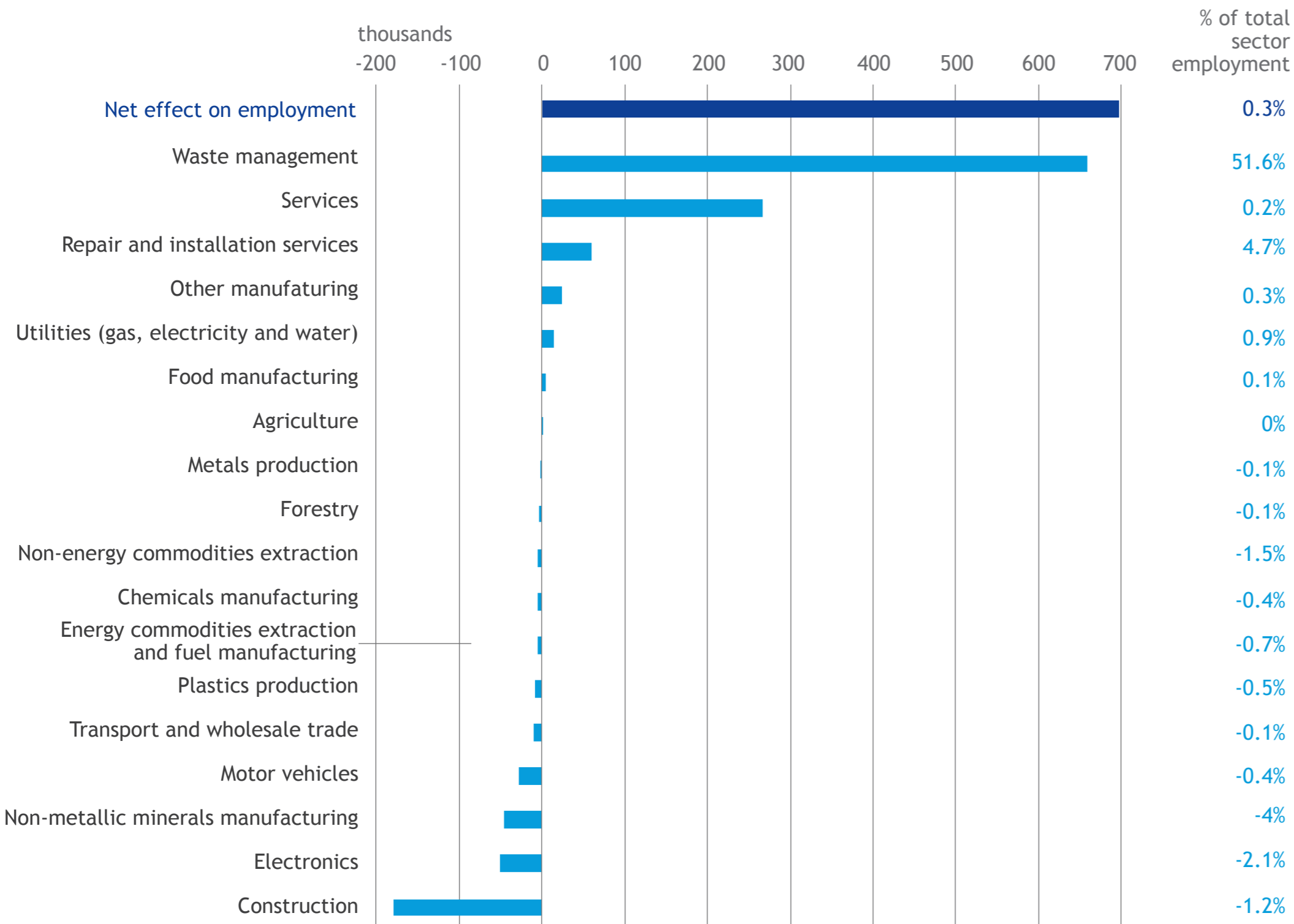
CHART 2. CHANGE IN EMPLOYMENT BETWEEN 2015-2030 DUE TO INTRODUCING OF A CIRCULAR ECONOMY
